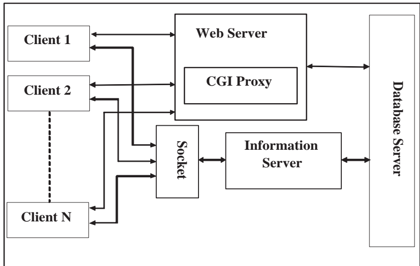
Fig. 1. TerraFly system architecture.
