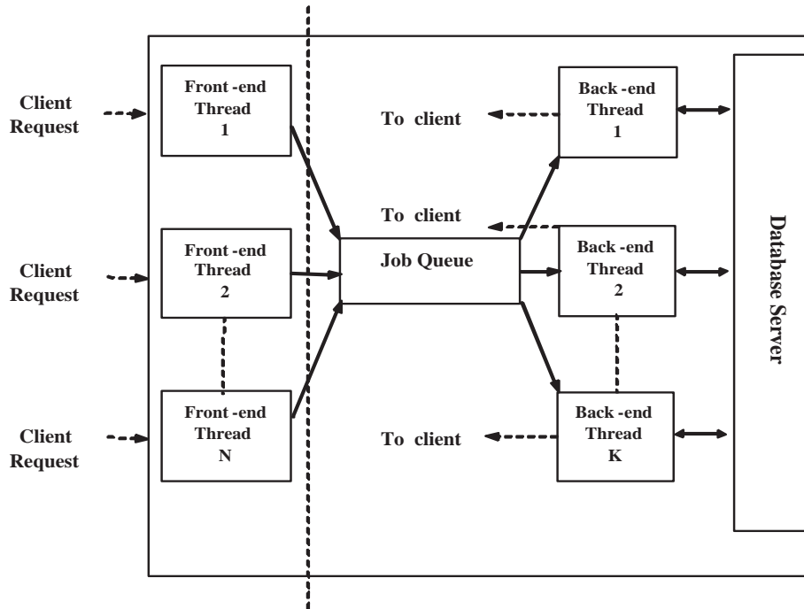
Fig. 4. The Internally Distributed Multithreading (IDMT) model design.
