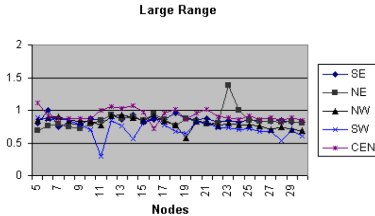
Fig. 10. Range query results with large size range.
