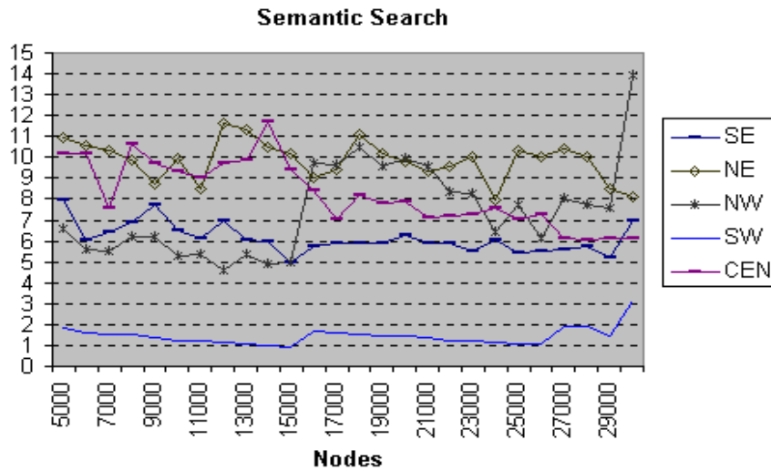
Fig. 12. Results of finding all objects with category “Bank.”
