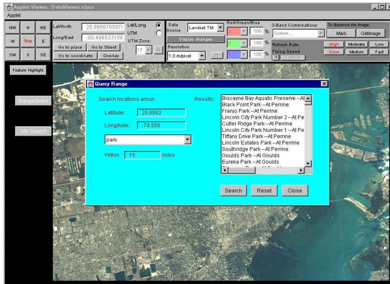
Fig. 6. Range query searching and its results listed in Results List Box.
