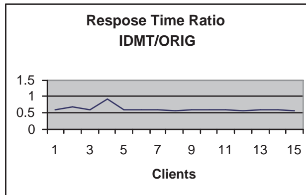
Fig. 9. Relative response time in the case of multiple clients.
