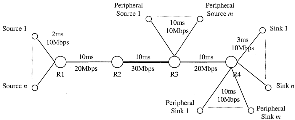
Fig. 4. Network topology with multiple bottlenecks and cross-traffic.
