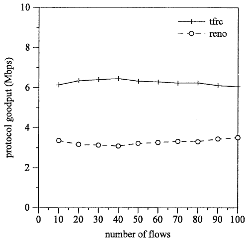
Fig. 25. TFRC competing with and Reno flows (10 Mbps bottleneck link).
