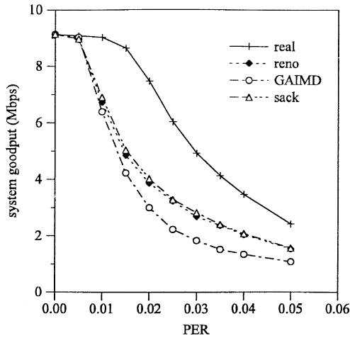
Fig. 13. Goodput over heterogeneous network (10 Mbps bottleneck link, 10 flows).
