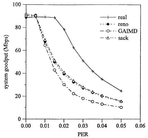
Fig. 14. Goodput over heterogeneous network (100 Mbps bottleneck link, 100 flows).
