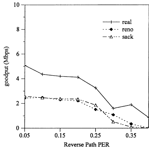
Fig. 20. Goodput over asymmetric path (10 Mbps bottleneck link, single flow forward path PER 0.001).
