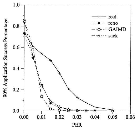
Fig. 18. 90% application success percentage (10 Mbps bottleneck link, 10 flows).
