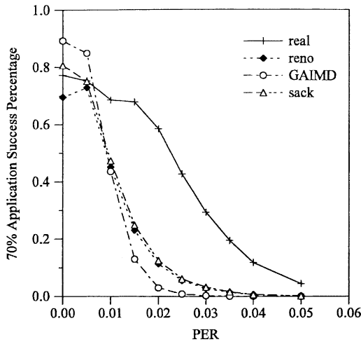
Fig. 19. 70% application success percentage (100 Mbps bottleneck, 10 Mbps wireless link, 100 flows).
