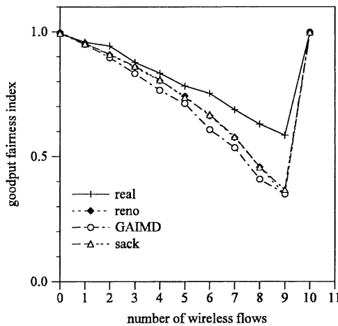
Fig. 16. Fairness with wired and wireless flows (10 Mbps bottleneck, PER = 0.01, 10 flows).
