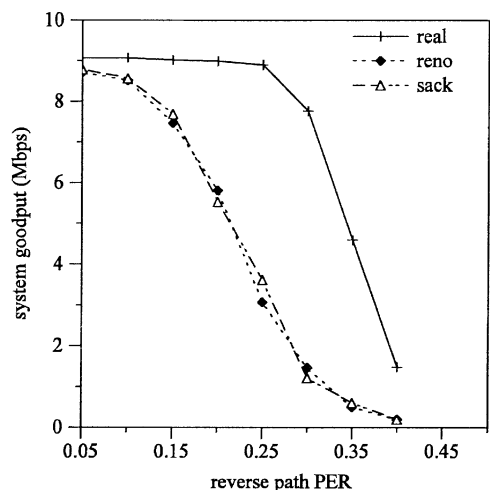
Fig. 21. Goodput over asymmetric path (10 Mbps bottleneck link, 10 flows 0.005 forward path PER).
