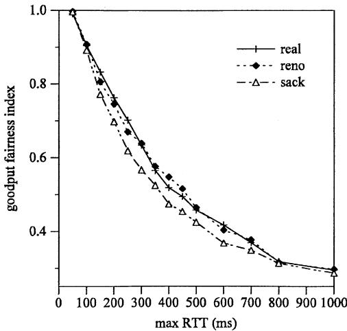
Fig. 8. Fairness over wired network (100 Mbps bottleneck link, 50 flows. RTTs are uniformly distributed between 30 ms and max RTT).
