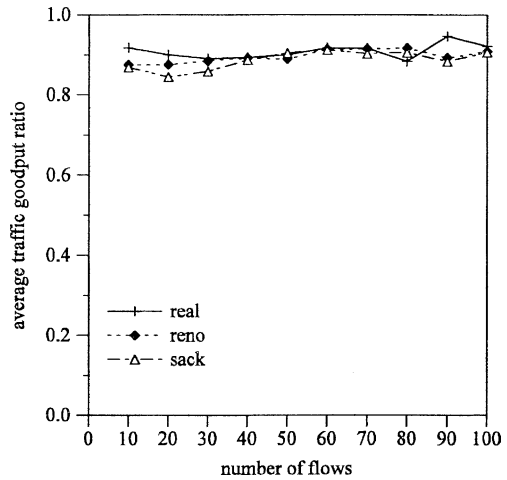
Fig. 10. Traffic goodput ratio over wired network (multiple bottlenecks, with RED gateways).
