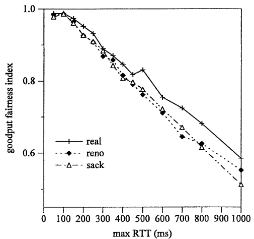
Fig. 7. Fairness over wired network (10 Mbps bottleneck link, 50 flows. RTTs are uniformly distributed between 30 ms and max RTT).
