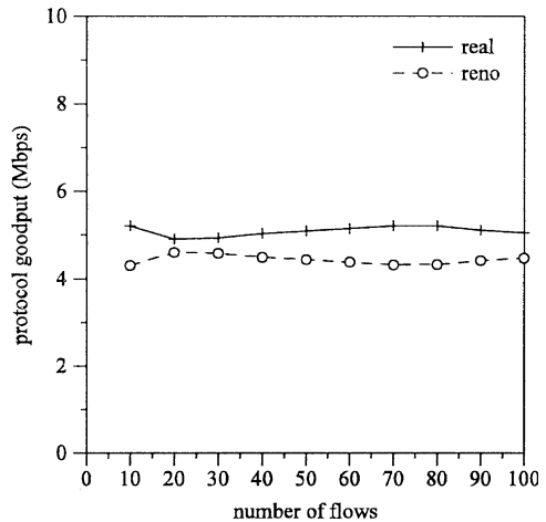
Fig. 24. Real competing with and Reno flows (10 Mbps bottleneck link).
