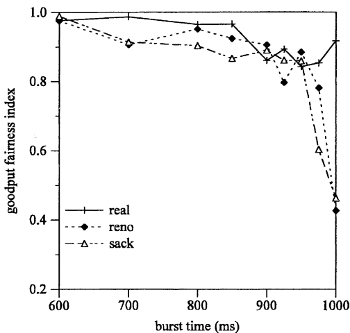
Fig. 23. Fairness over wired network (multiple bottlenecks, 5 flows of main traffic reverse path congested by cross-traffic).
