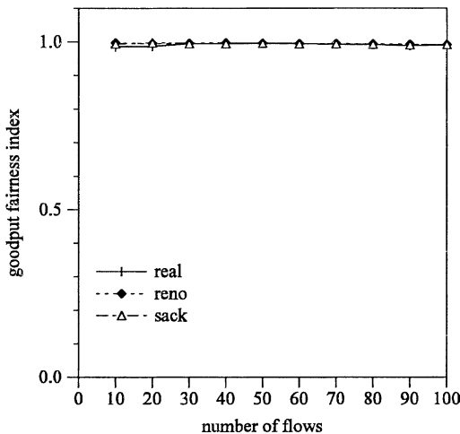
Fig. 6. Fairness over wired network (10 Mbps bottleneck link).
