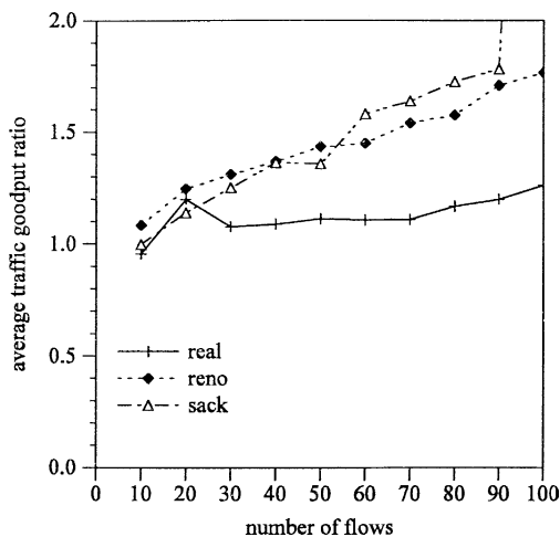
Fig. 9. Traffic goodput ratio over wired network (multiple bottlenecks, with drop tail gateways).
