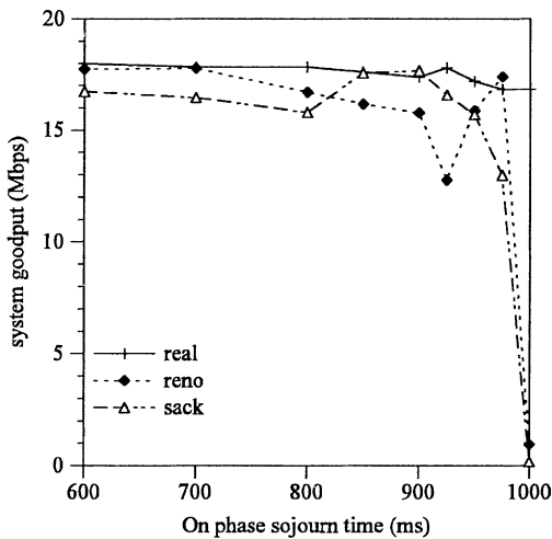
Fig. 22. Goodput over wired network (multiple bottlenecks, 5 flows of main traffic reverse path congested by cross-traffic).
