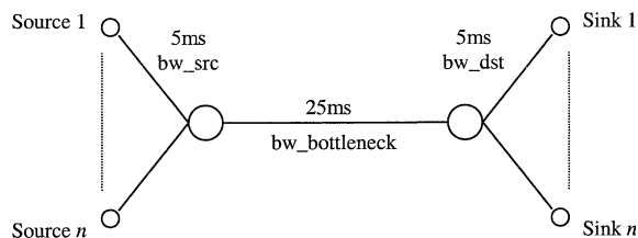
Fig. 3. Dumbbell network topology.
