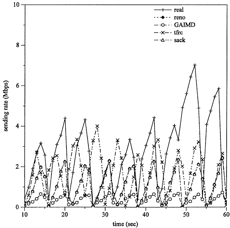
Fig. 12. Sending rate with handoff (10 Mbps bottleneck link, single flow).
