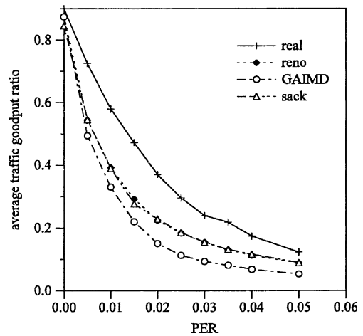
Fig. 17. Traffic goodput ratio over heterogeneous networks (multiple bottlenecks, 20 flows).
