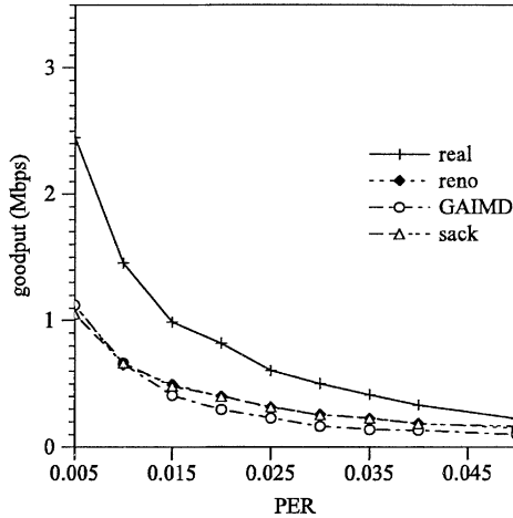
Fig. 11. Goodput over heterogeneous network (10 Mbps bottleneck link, single flow).
