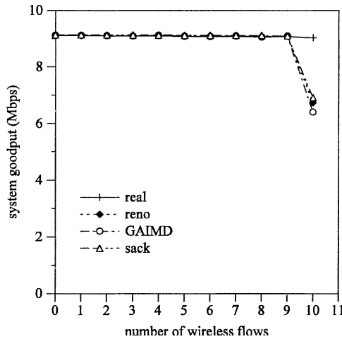
Fig. 15. Goodput with wired and wireless flows (10 Mbps bottleneck, PER = 0.01, 10 flows).
