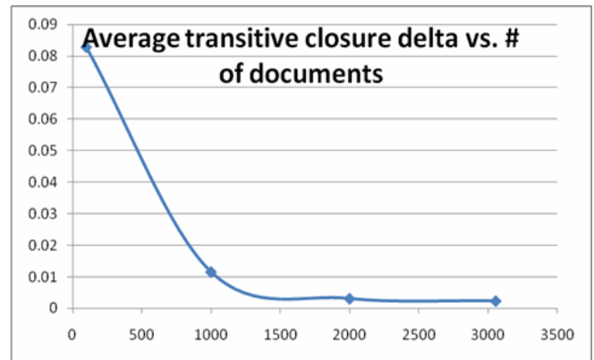
Figure 6. Contribution of Transitive Closure diminishes for large document corpuses.
