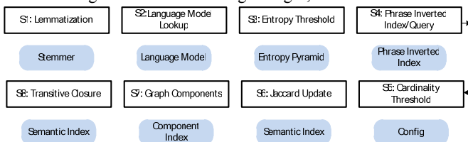
Figure 3. SPSI mining algorithm: Stages S1-S8 and data structures that go with them.
