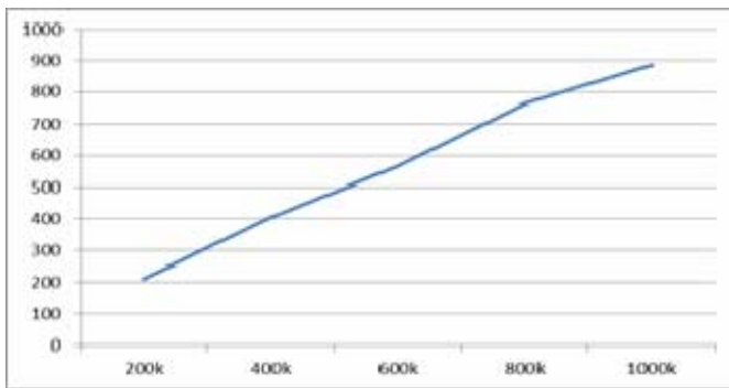
Figure 7. Total execution time in seconds versus total number of documents.
