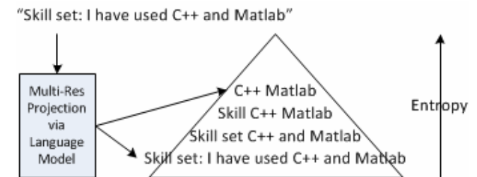
Figure 4. Entropy sliced pyramid structure. Each level contains all terms at or above the entropy threshold for that level. We may decide to truncate the pyramid at some level if we only need it for semantic indexing, otherwise we go all the way to the bottom for full text indexing.
