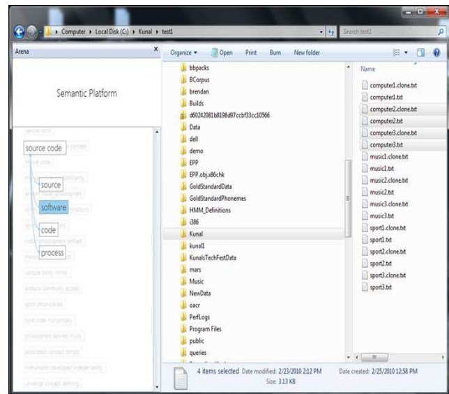
Figure 9. Exploring mined concepts in a file system. When a concept is browsed on the left, the corresponding files are highlighted on the right.
