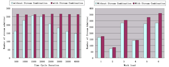
(a) Varying time-cycle duration.
