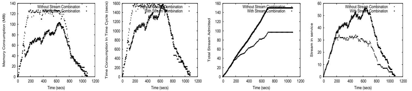
Figure 6: Comparison for time-cycle=5000ms.
