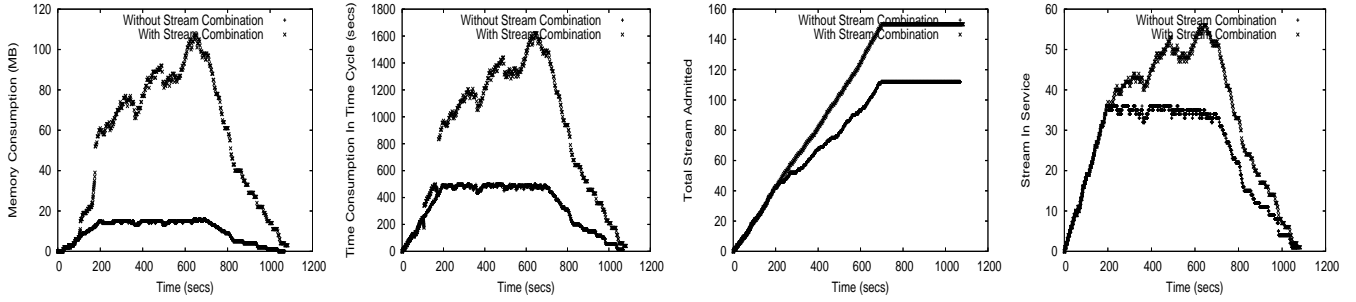
Figure 5: Comparison for time-cycle=500ms.
